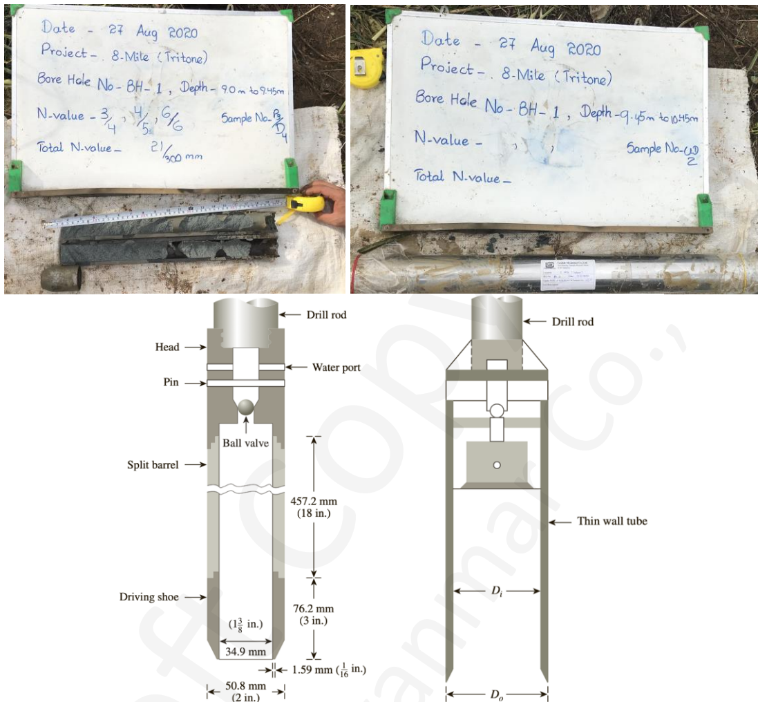
Figure 63: Sample Collection with Split Spoon Sampler and Thin Wall Tube
