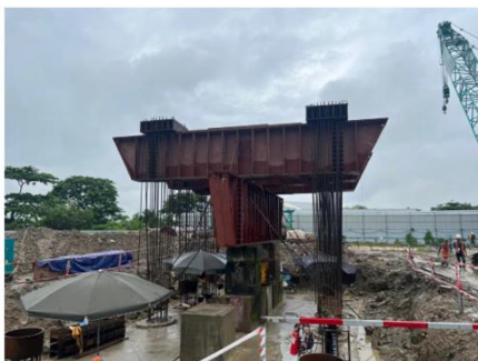
Pile Static Load Test
