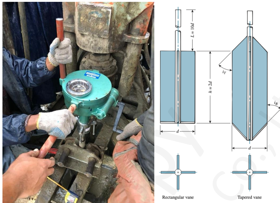
Figure 64: Vane Shear Testing Photos
