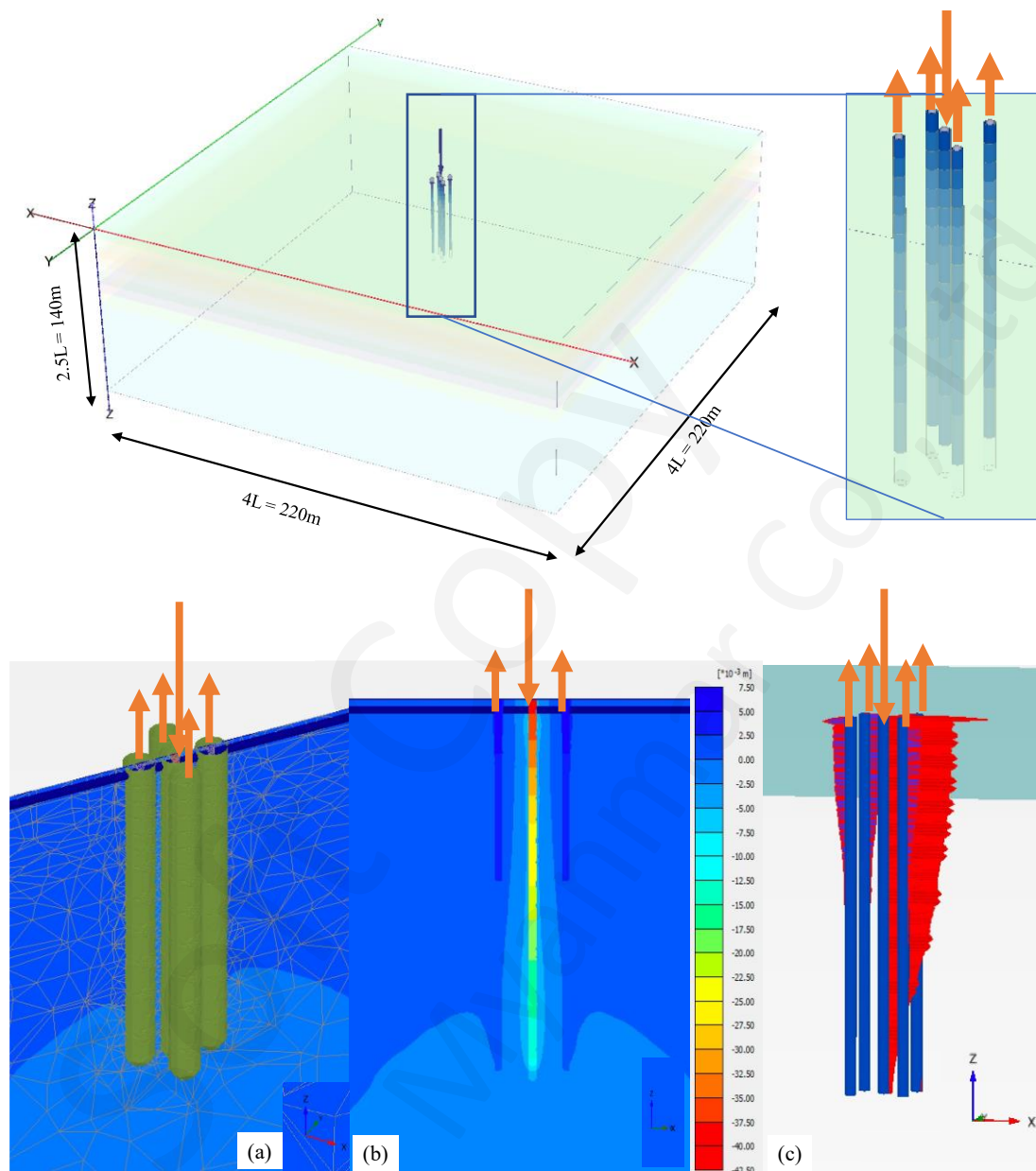
Figure 89: Pile Test FEM model for Research
