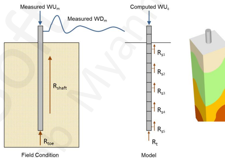
Figure 10: Wave Equation Analysis Concept, Allwave DLT Program
