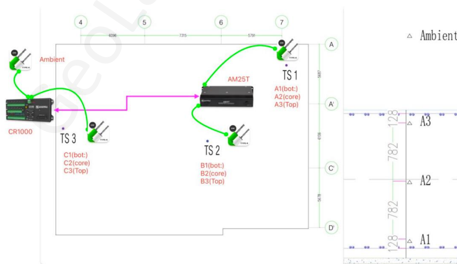
Figure 39: Temp Measuring Plan in Mass Concreting
