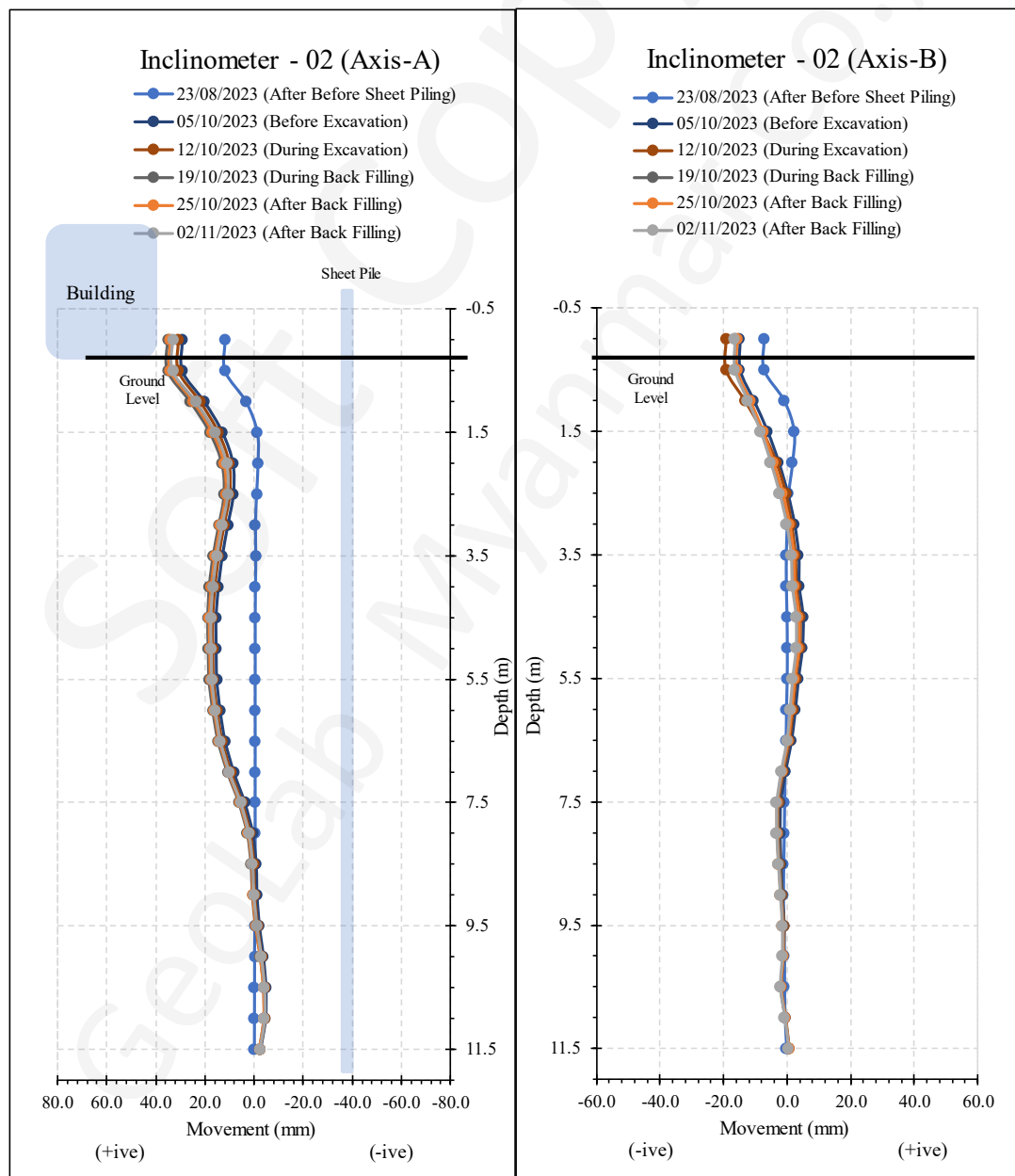
Figure 27: ERSS, TERS Inclinator Monitoring Result Sample
