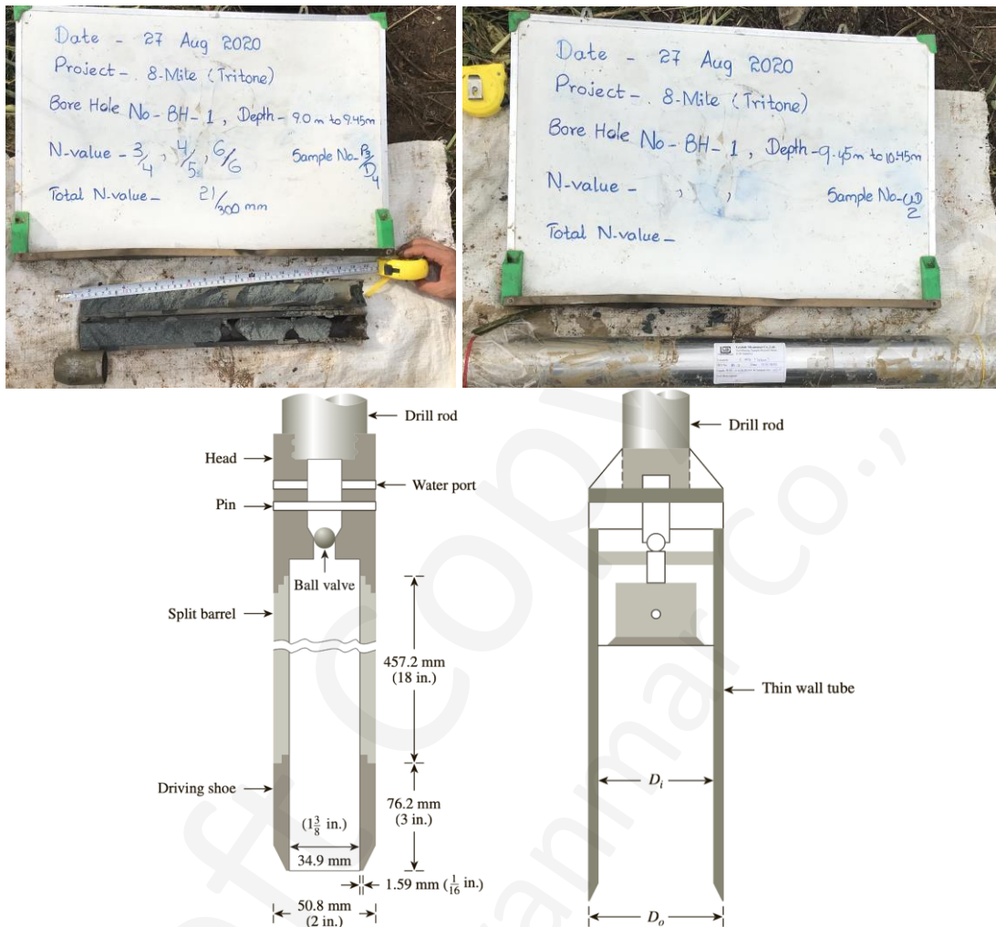
Figure 63: Sample Collection with Split Spoon Sampler and Thin Wall Tube
