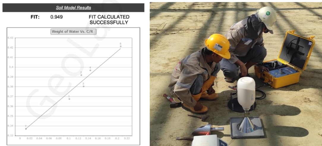
Figure 24: EDG Tests Soil Model Building with Sand Cone Test
