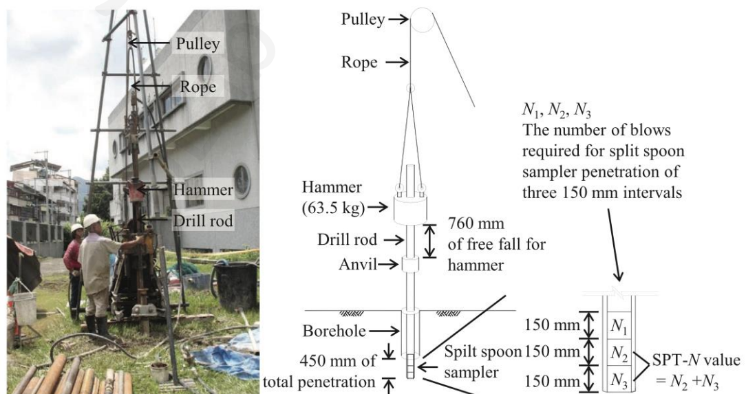
Figure 62: SPT Testing at Site
