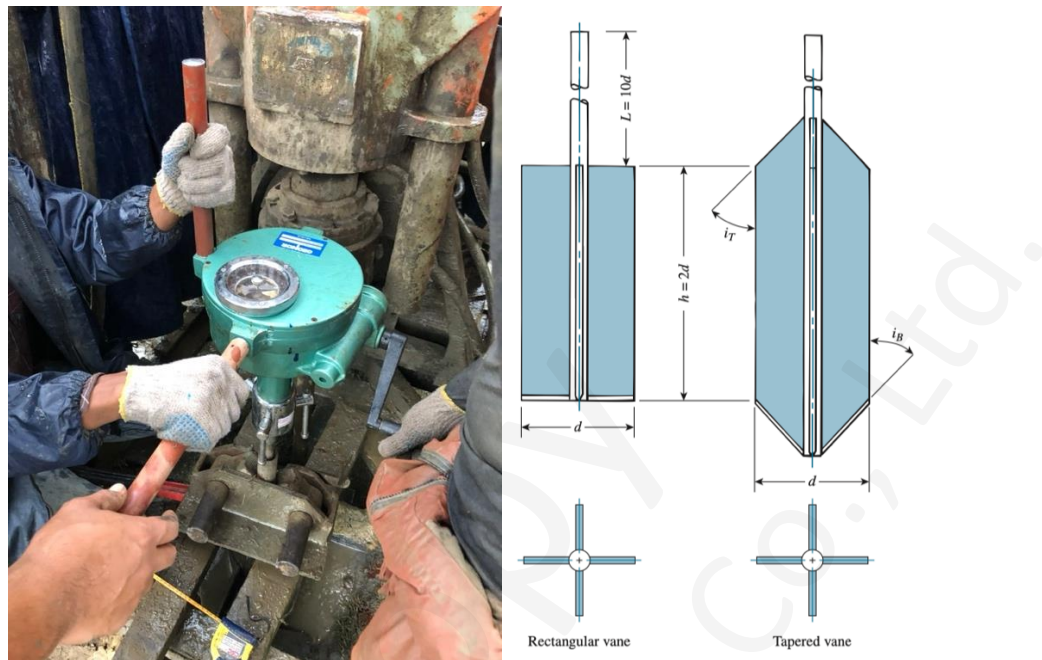
Figure 64: Vane Shear Testing Photos
